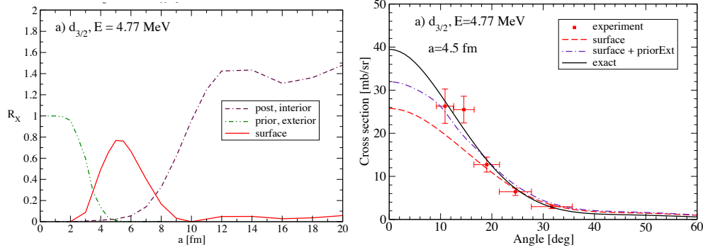
Fig. 2: Examination of interior, surface, and exterior contributions for transfers to resonance states in ^{21}\text{O} , for the 3/2^+ resonance at 4.77 MeV. The left panel shows the interior (post) term, the surface term, and the exterior (prior) term, as a function of the surface radius. The right panel shows that improvements to the surface-term-only approximation can be achieved by including contributions from the prior-exterior term and selecting a small surface radius. The potential V_{nA} , which binds the neutron to the ^{20}\text{O} nucleus, has a radius of 3.39 fm and a diffuseness of 0.65 fm.
